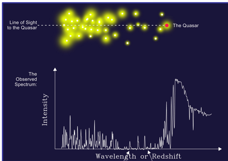
the intergalactic-medium
