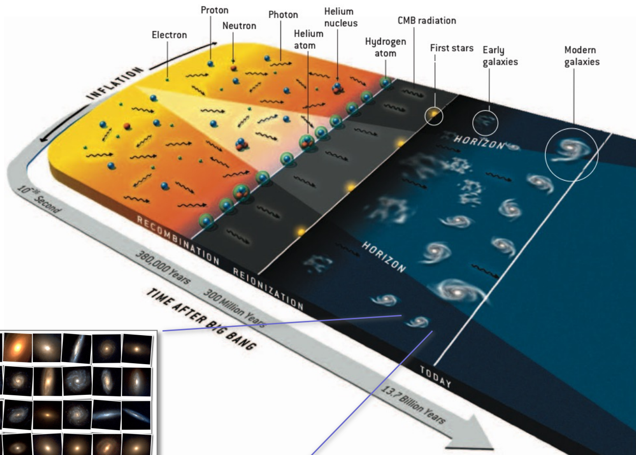
the galaxy zoo
