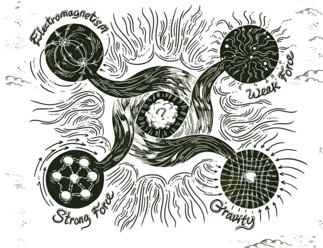
physics of the early Universe
