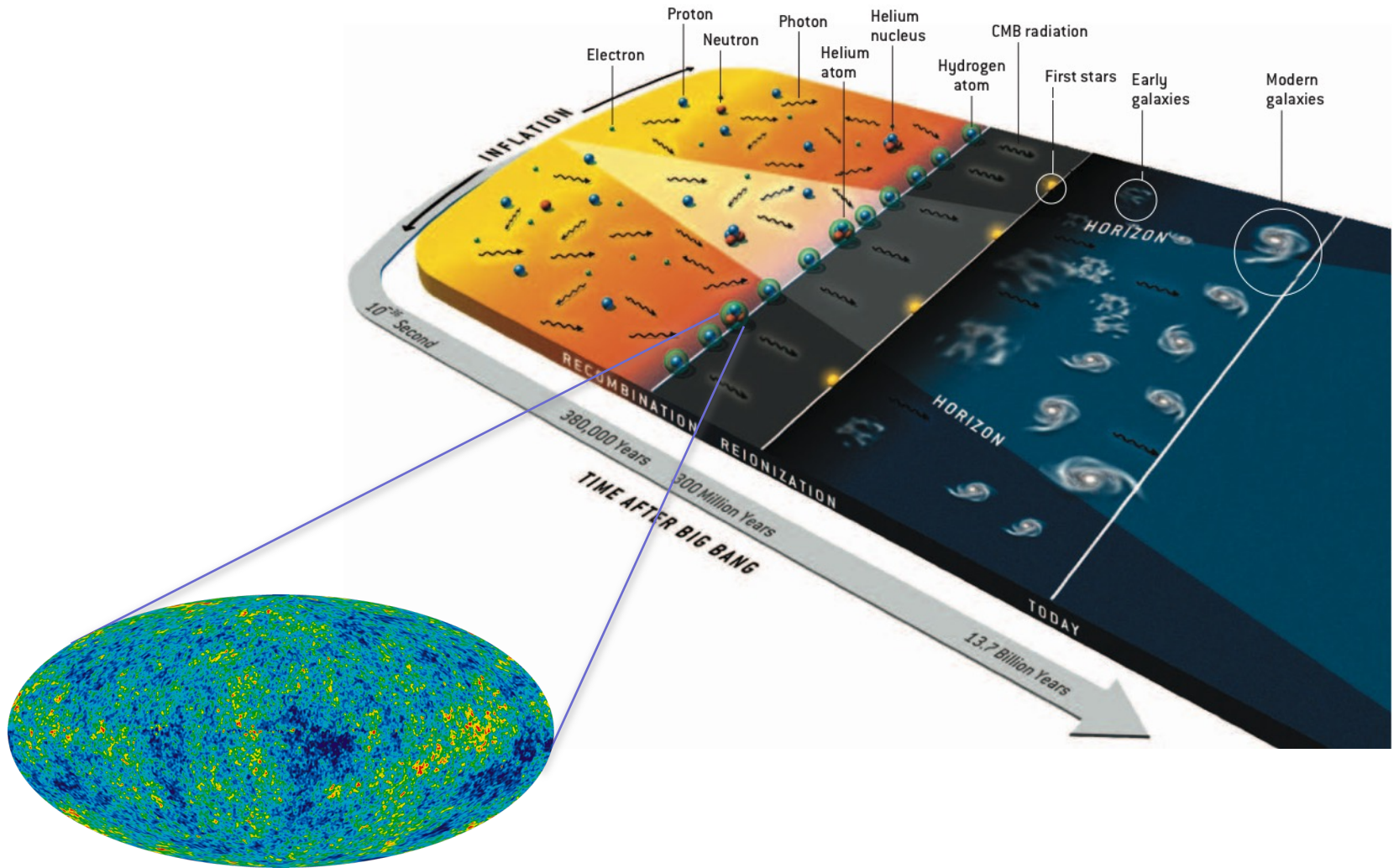
cosmic microwave background radiation
