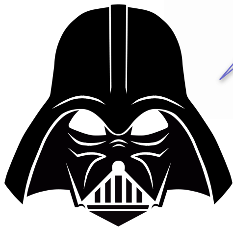
the dark ages
