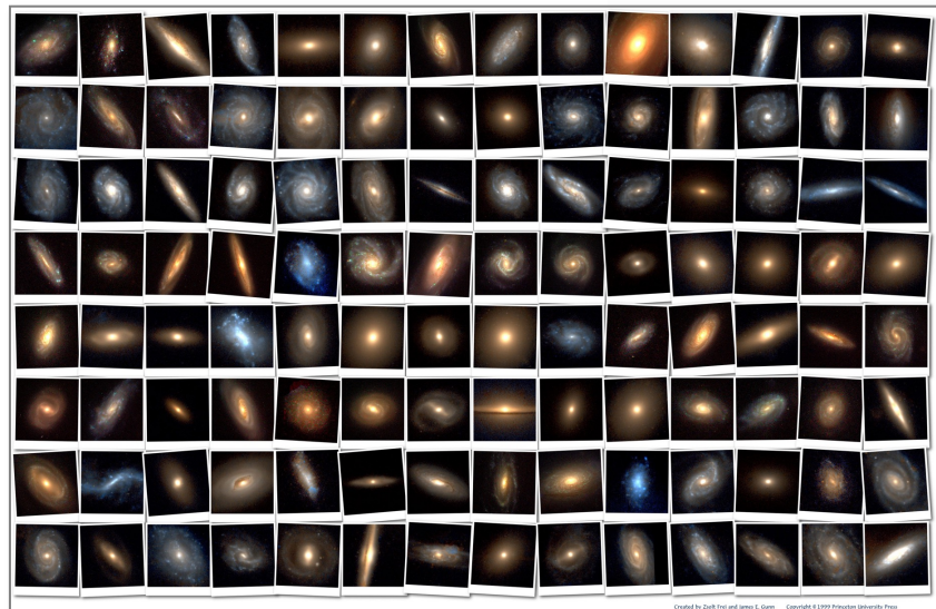
the galaxy zoo
