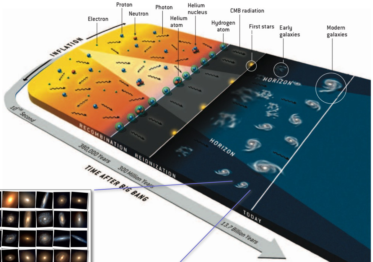
the galaxy zoo
