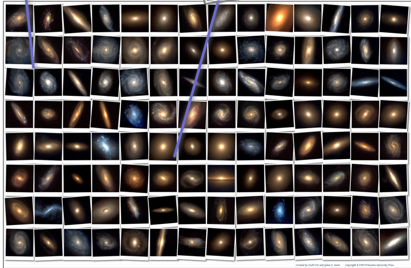
the galaxy
